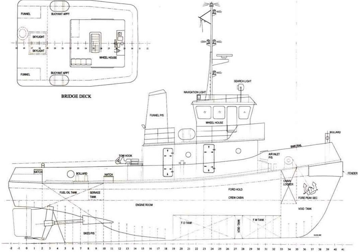
MAIN PROFILE
