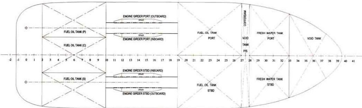
BOTTOM PLAN
