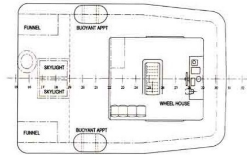
BRIDGE DECK
